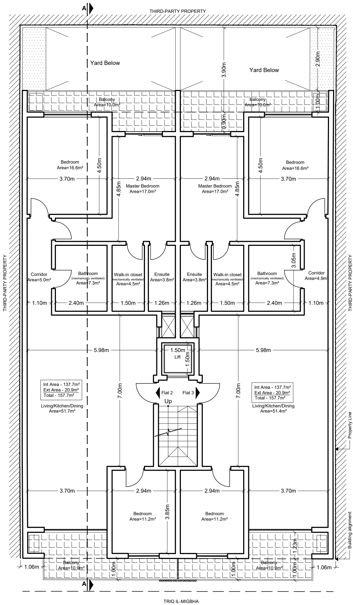
PROPOSED FIRST FLOOR Scale 1:100
