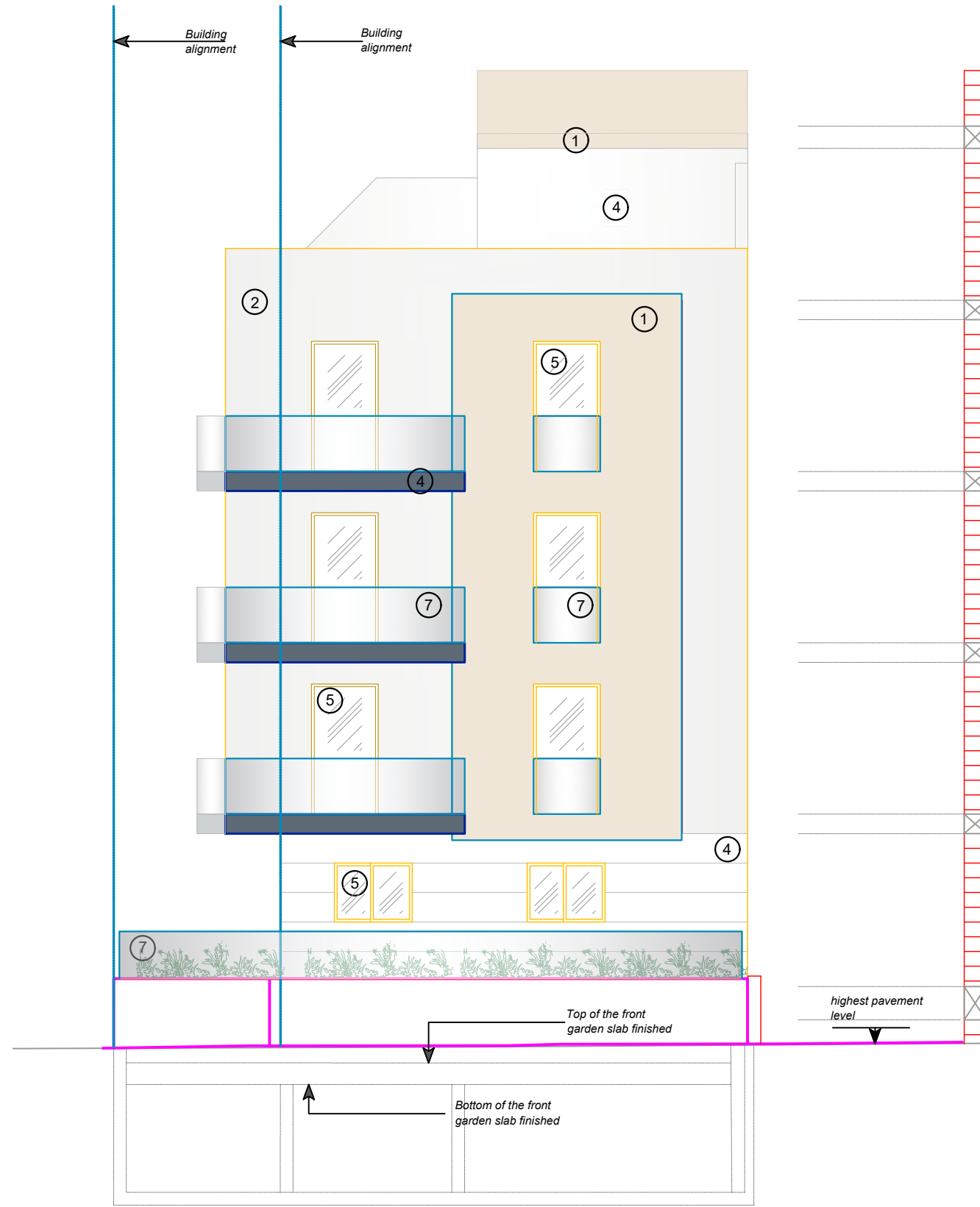
Proposed side elevation scale 1:100
